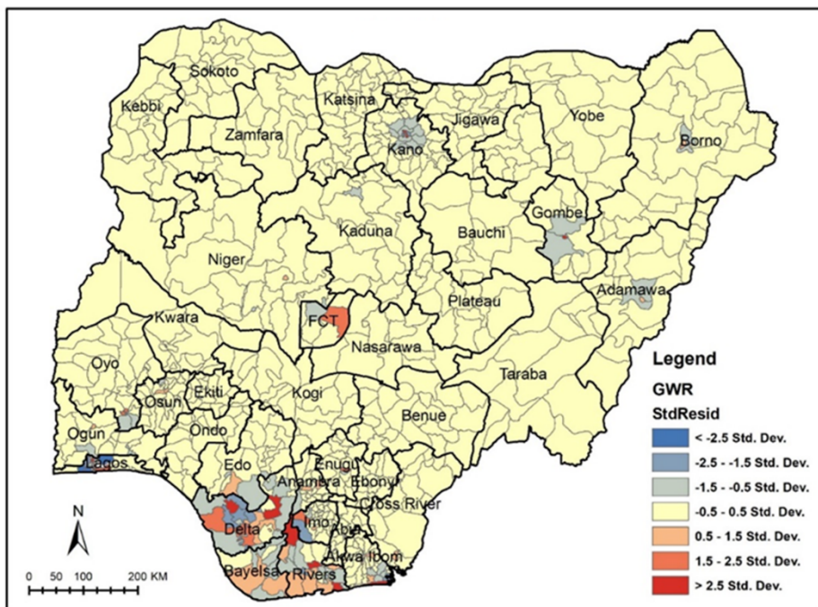
Figure 1. GWR - Standard Residual Map
